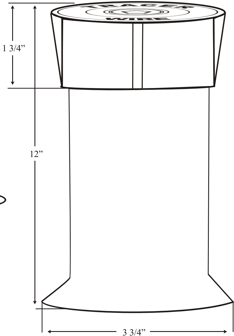
Figure # TRAB Tracer Wire Access Box
