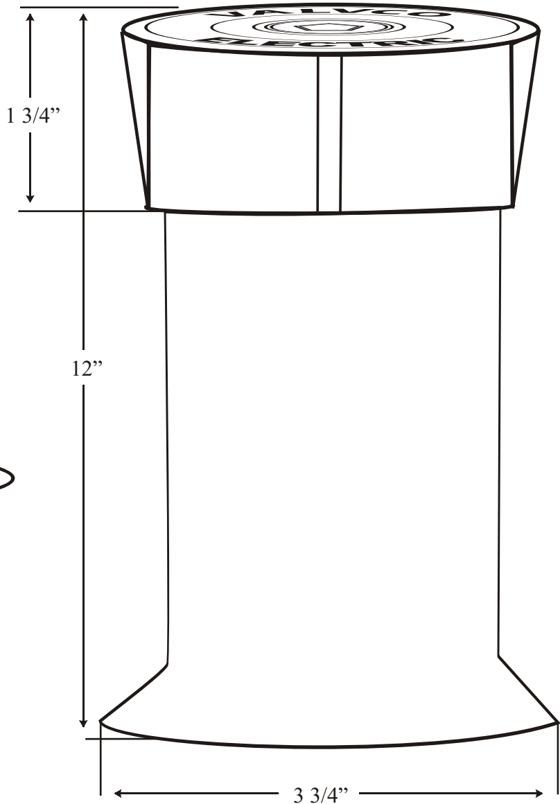
Figure # ELAB Electric Tracer Wire Access Box
