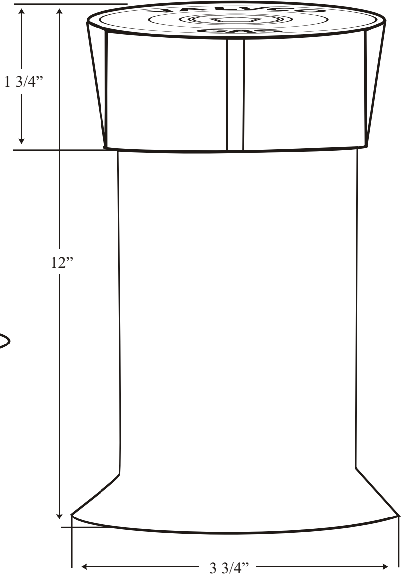
Figure # GAB Gas Tracer Wire Access Box
