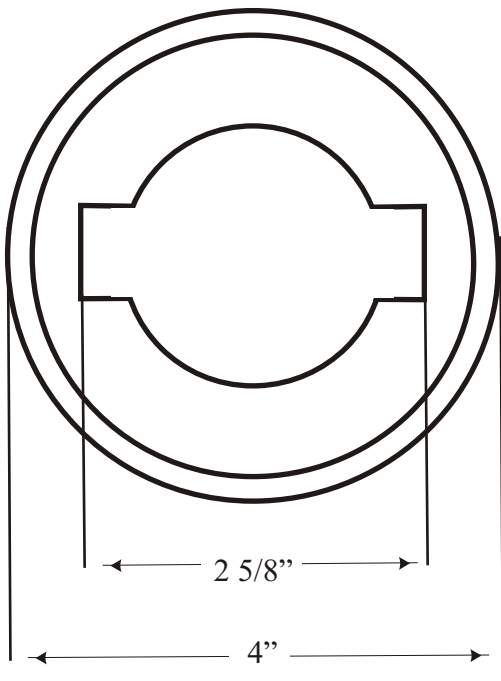
Collar Top View
