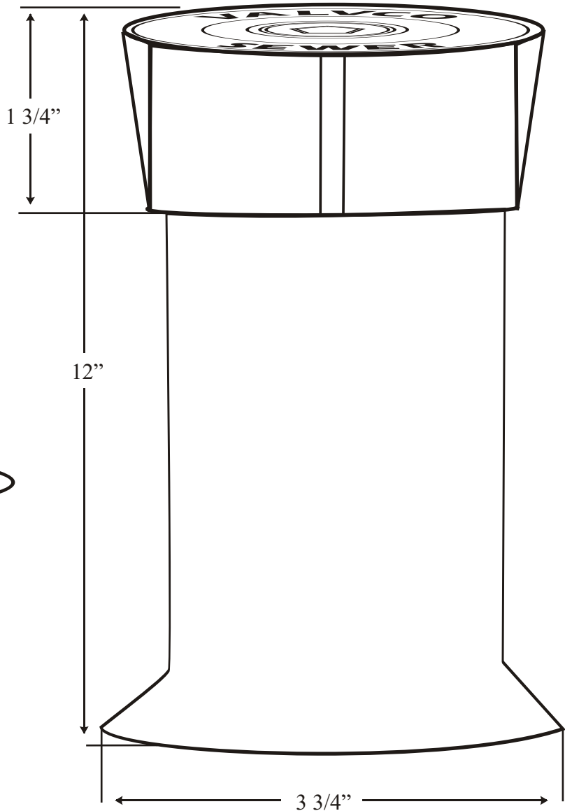
Figure # SEWAB Sewer Tracer Wire Access Box
