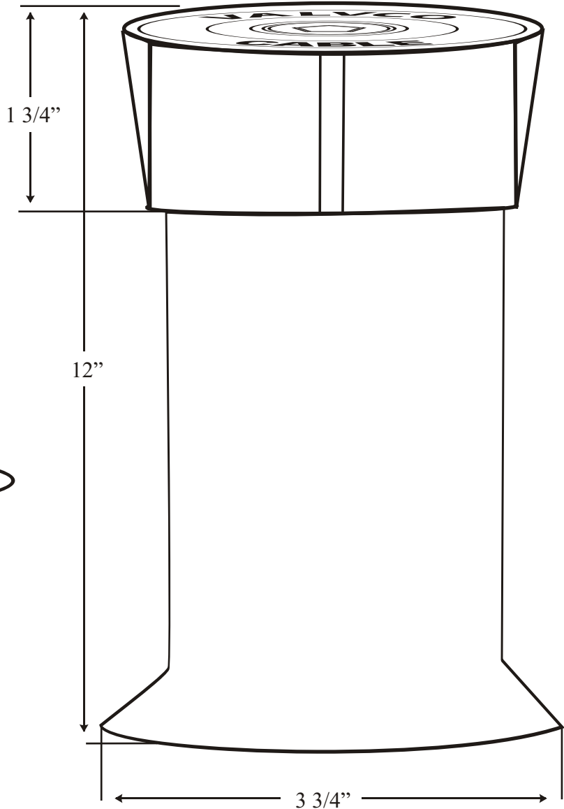
Figure # CAB Cable Tracer Wire Access Box
