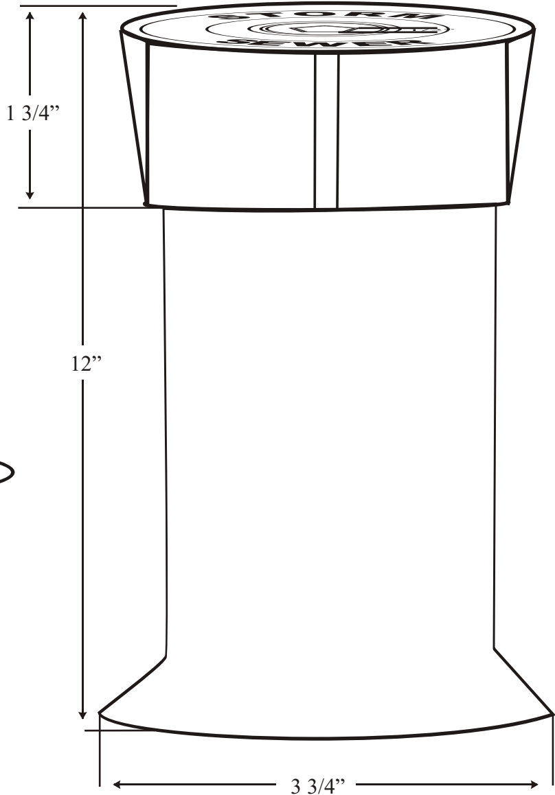
Figure # SSAB Storm Sewer Tracer Wire Access Box
