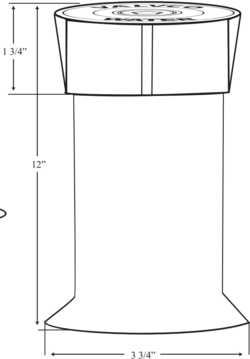
Figure # TWAB Water Tracer Wire Access Box
